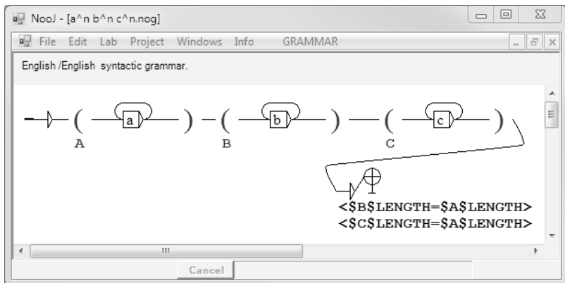
Figure 3: Context-Sensitive Grammar
